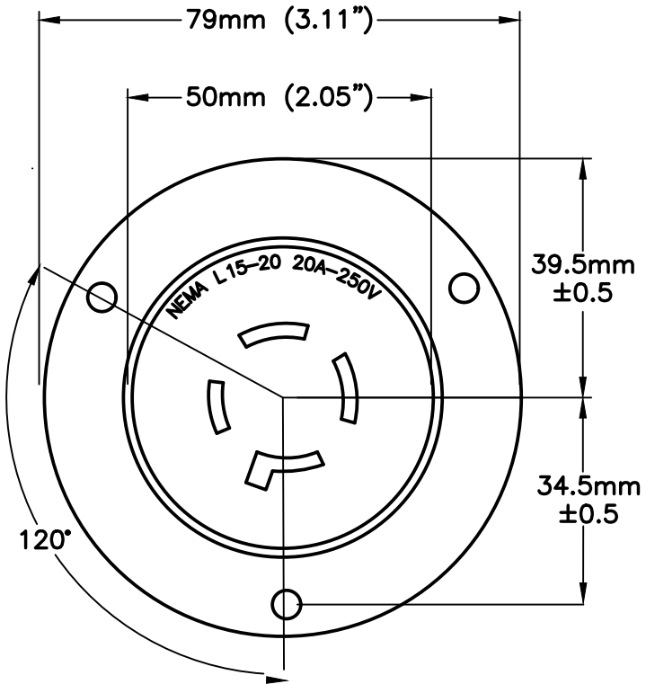
NEMA L15-20 RECEPTACLE FRONT VIEW
